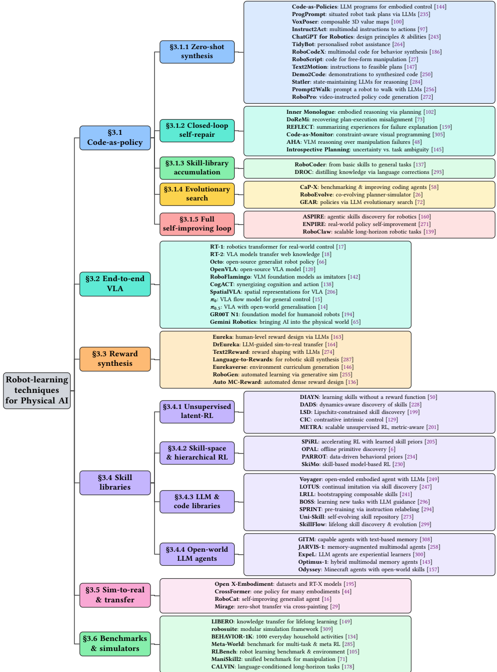
Fig. 1. The weights-versus-skills taxonomy of robot learning (all 77 systems). Each sub-family is one cell listing its systems, each with a trimmed form of the paper’s own title. Left fork = inspectable code / skills (§3.1, §3.4); the §3.1 cells are shaded by degree of self-improvement , from zero-shot to the full feedback+memory+search loop. Full per-system detail: Tables 2–6.
