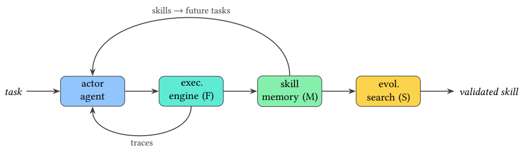
Fig. 3. The full self-improving loop (§3.1.5): feedback (F) + memory (M) + search (S) combine into one open-ended loop (occupied by ASPIRE, ENPIRE, and RoboClaw). VLAs (§3.2) have no such loop.
