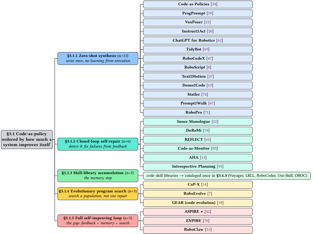
Fig. 3. The self-improvement funnel within code-as-policy ( 13 \rightarrow 6 \rightarrow 5 \rightarrow 3 \rightarrow 3 ), one colour per sub-section. As the demand rises (write once \rightarrow repair \rightarrow remember \rightarrow search \rightarrow all three), occupants thin out; §3.1.5—feedback + memory + search combined—is nearly empty, and only ASPIRE ★ was built for it end-to-end.
