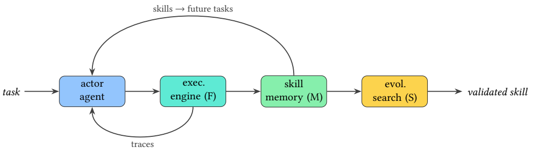
Fig. 4. The full self-improving loop (§3.1.5): feedback (F) + memory (M) + search (S) combine into one open-ended loop—the ASPIRE cell. VLAs (§3.2) have no such loop.
