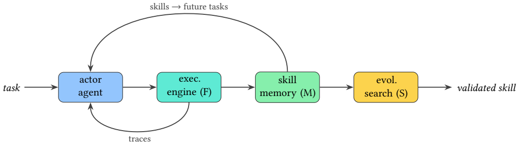
Fig. 3. The full self-improving loop (§3.1.5): feedback (F) + memory (M) + search (S) combine into one open-ended loop (occupied by ASPIRE, ENPIRE, and RoboClaw). VLAs (§3.2) have no such loop.
