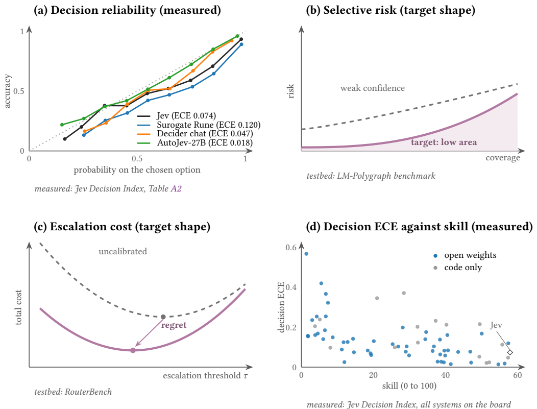
Fig. 11. A measurable agenda, partly measured. Decision ECE is the expected calibration error of the probability a model places on its chosen option (Table 6). Panels (a) and (d) come from one community leaderboard, the Jev Decision Index [multimodalart 2026] (release 0.2.1, a single snapshot of 2026-09-27; not peer reviewed): skill is its chance-normalised score over 38 decision benchmarks (0 to 100), ECE is computed on a 1-in-6 sample of 32 of them, and all values are point estimates without uncertainty intervals. (a) Reliability measured on the Jev Decision Index (Table A2) for Jev and the three open systems with the highest skill; each point is a confidence bin, and bins holding under 1% of answers are omitted. (b) Selective risk and (c) escalation regret are drawn as target shapes, not measured results: purple marks the target, grey dashed a typical baseline, and the named testbeds are in Table 6. (d) Decision ECE against skill for Jev and the 67 open systems on the board; lower right is better. The board records no cost per decision, so skill is used as the horizontal axis.
