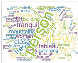
VBench arXiv:2311.17982
