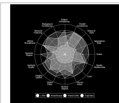
VBench arXiv:2311.17982
