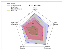
EvalCrafter arXiv:2310.11440
