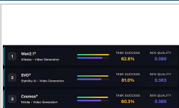
World-in-World arXiv:2510.18135
