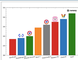
EvalCrafter arXiv:2310.11440
