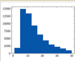
EvalCrafter arXiv:2310.11440
