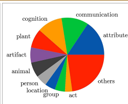
EvalCrafter arXiv:2310.11440
