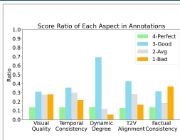
VideoScore arXiv:2406.15252
