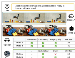
WorldModelBench arXiv:2502.20694
