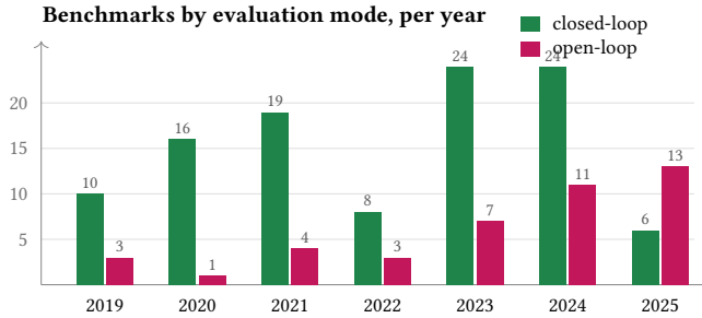
Fig. 2. The world-model-evaluation wave is recent. Per-year counts of closed-loop task-success benchmarks (green) and open-loop world-model / video-generation benchmarks (magenta) in the catalogue. Closed-loop suites dominate through 2024; in 2025 open-loop evaluation overtakes them (13 vs 6) as the world-model-generation literature arrives. The four prediction-to-action bridges are newer still, all appearing in 2024 or later. Years are the benchmarks’ first-release years (2026 is partial and omitted); counts are the tallies of Table ??.
