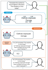
Fig. 8. How confidence is produced and used, by stage. Each panel shows a whole figure of the cited paper, reproduced under its CC BY licence; its label links to the paper. The selection rule and each panel's figure, page and licence are in Table E1. S0 read-off has no panel: no reusable figure passed the check (Table E1).
