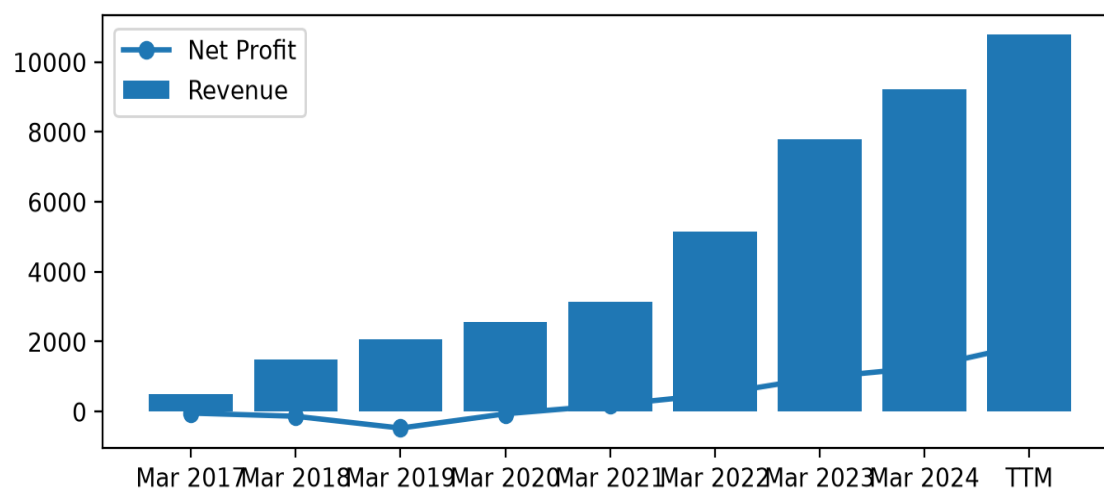
ADANIGREEN Revenue vs Net Profit
