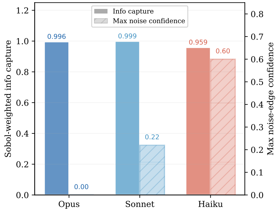
Discovery vs. false positives
