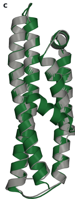
crystal structure and native model, 0.85 Å
