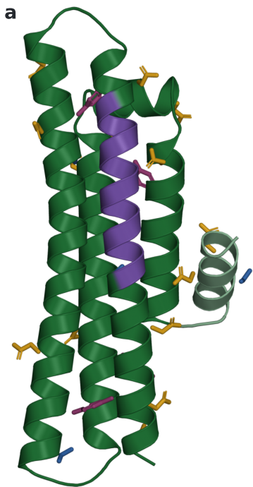
native fold, 22 converted positions
