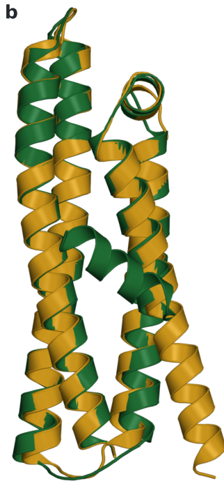
native and rQTY models, 0.71 Å over the bundle
