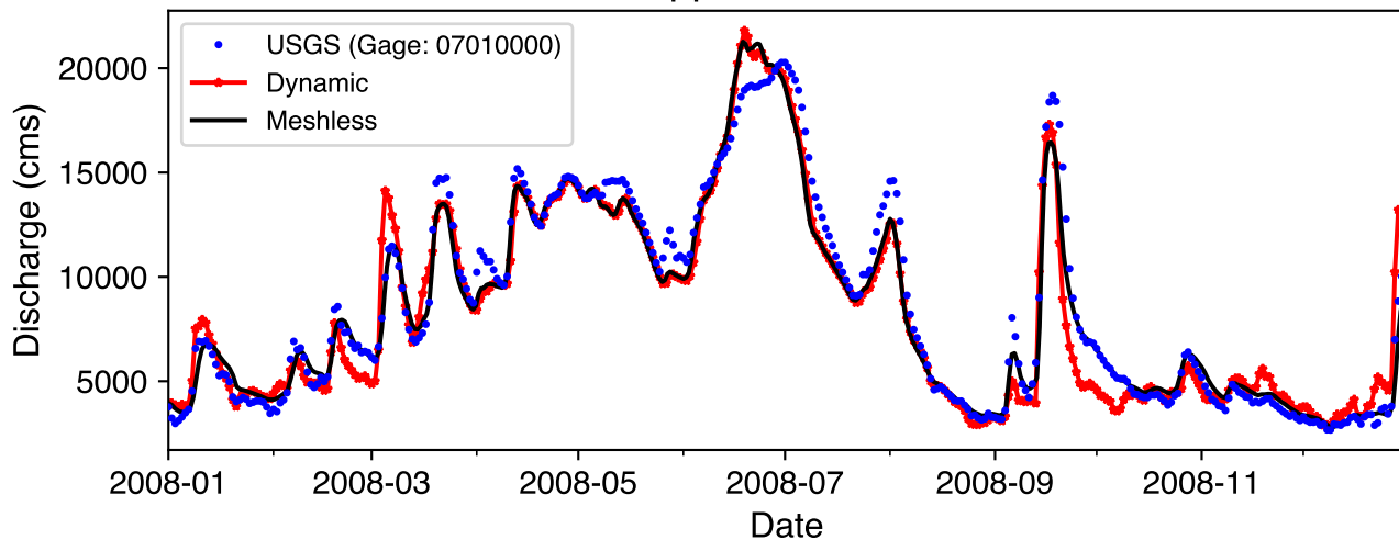
Mississippi River at St. Louis
