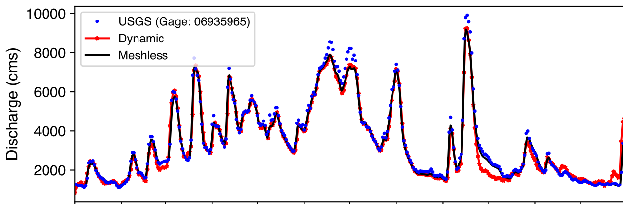
Missouri River at St. Charles
