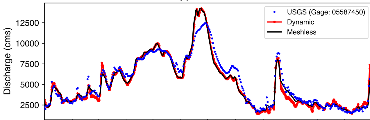
Mississippi River at Grafton
