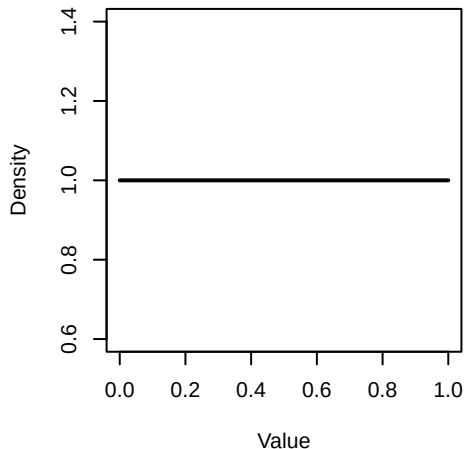
Uniform Distribution
