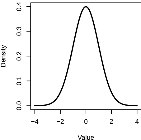
Normal Distribution
