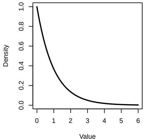
Exponential Distribution
