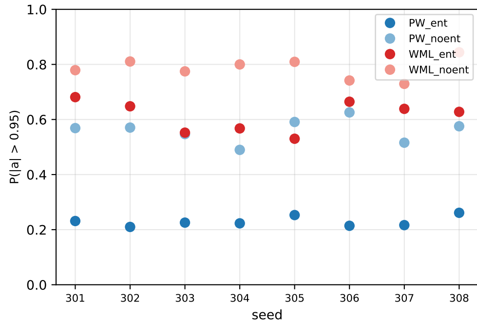
Walker entropy factorial: action saturation, per coordinate, frozen bank
