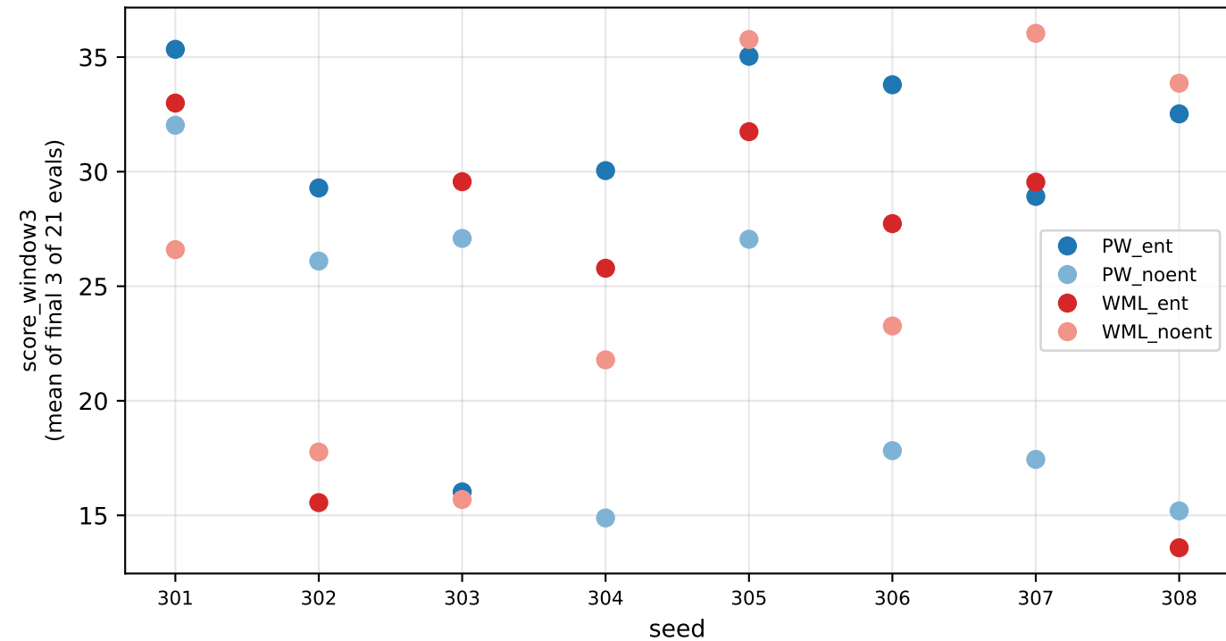
LeapCubeRotateZAxis entropy factorial: return, paired seeds
