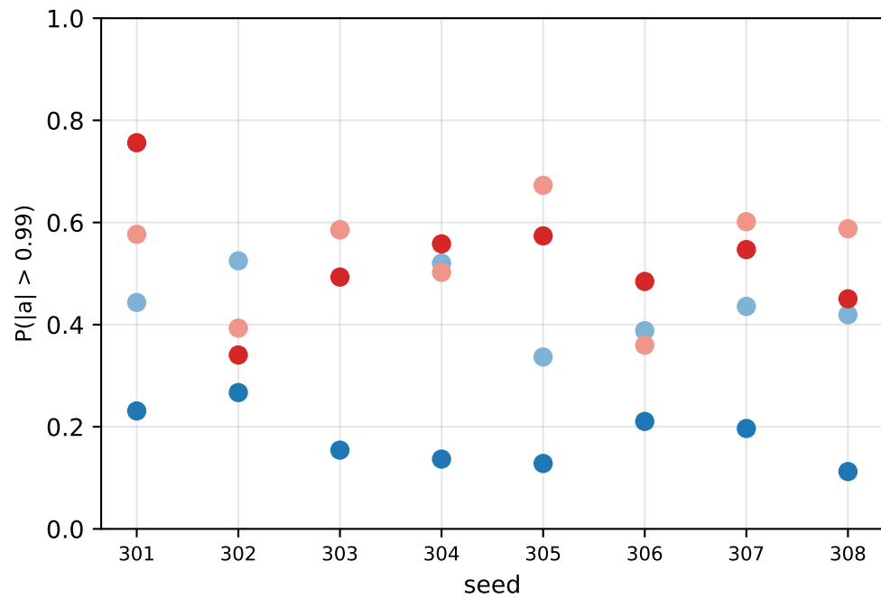
LeapCubeRotateZAxis entropy factorial: action saturation, per coordinate, frozen bank
