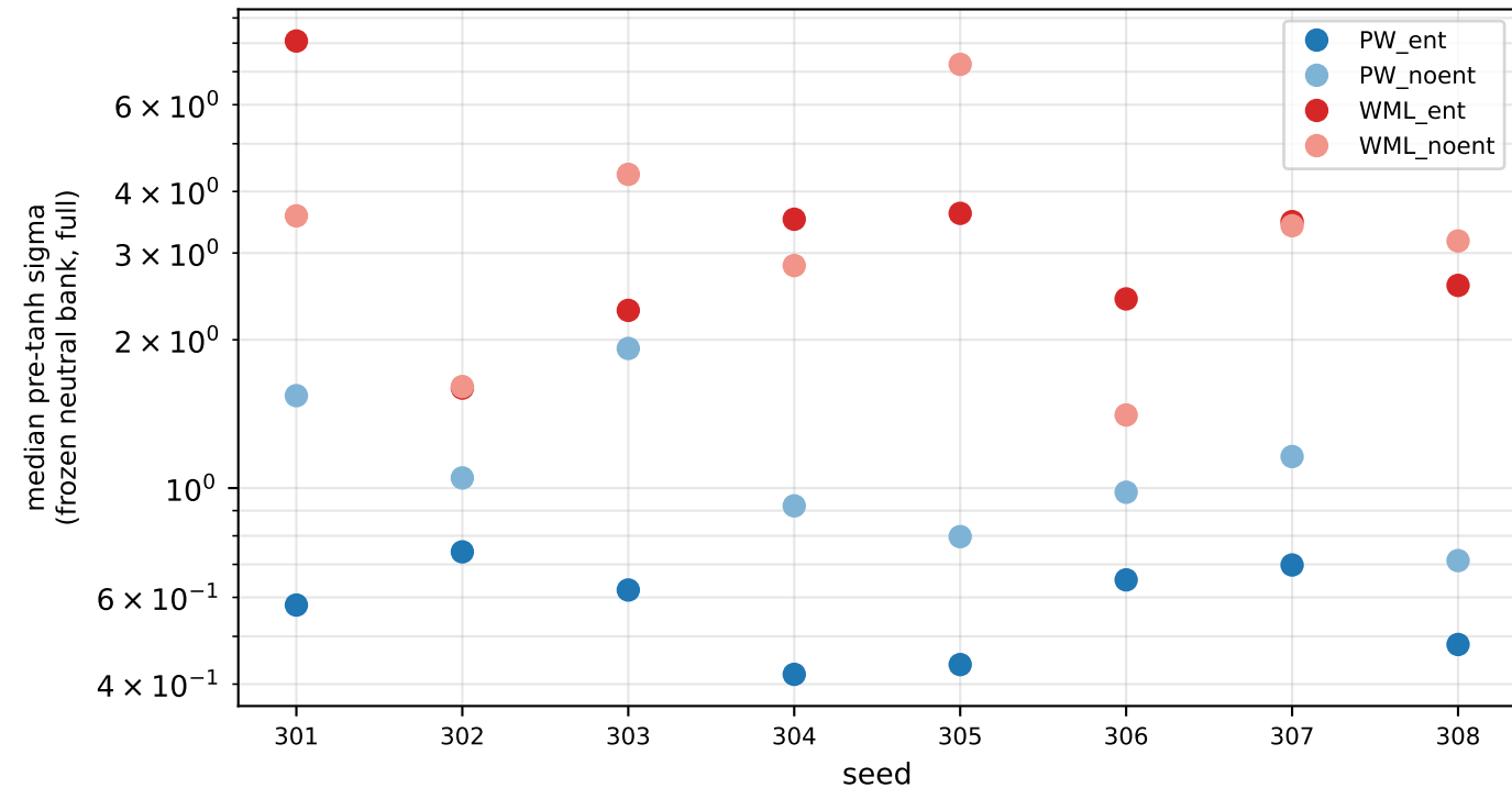
LeapCubeRotateZAxis entropy factorial: policy width, paired seeds
