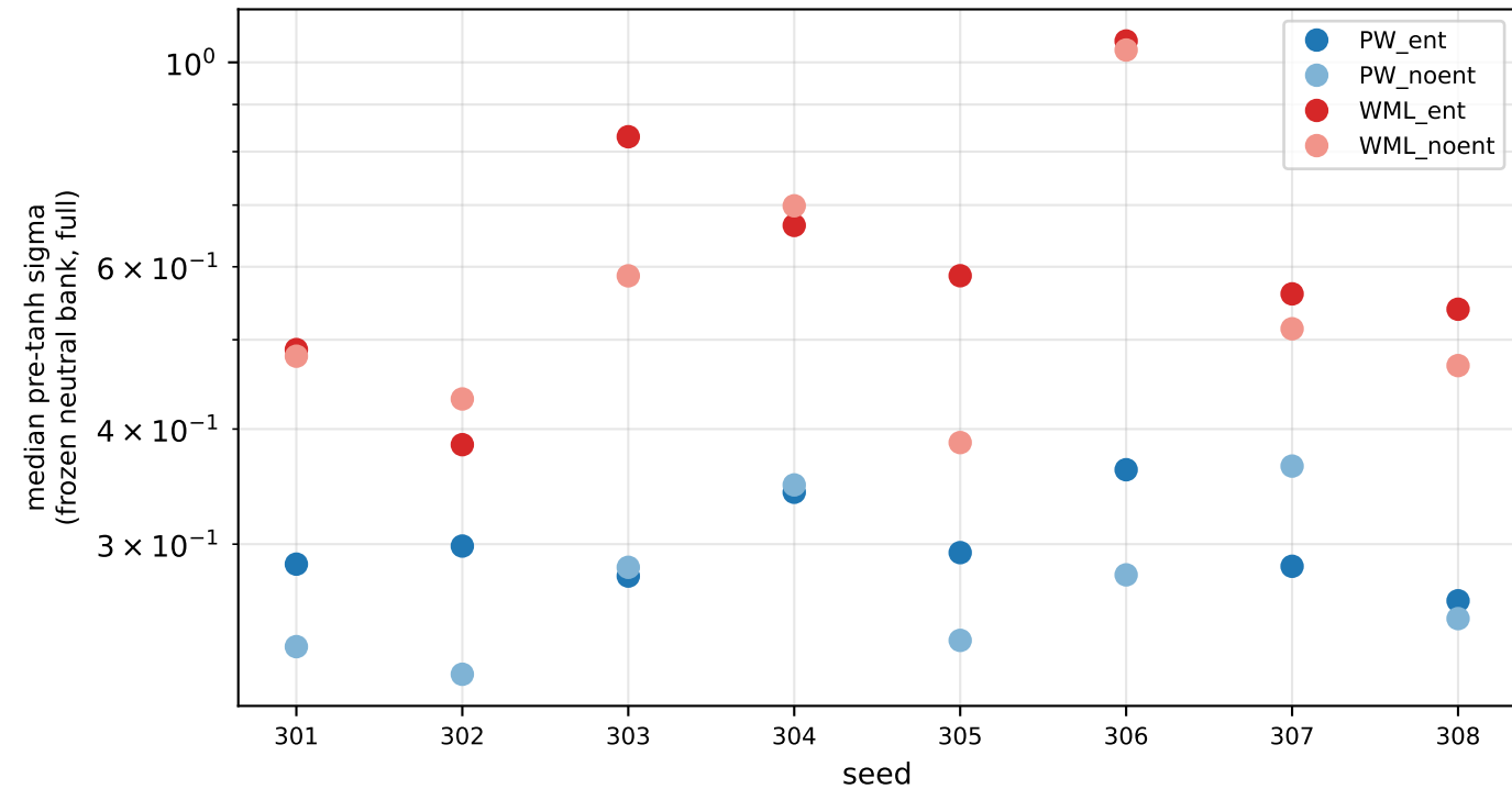
G1JoystickFlatTerrain entropy factorial: policy width, paired seeds
