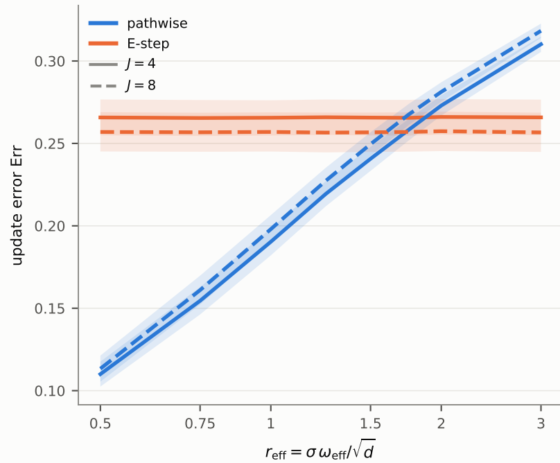
B Total update error
