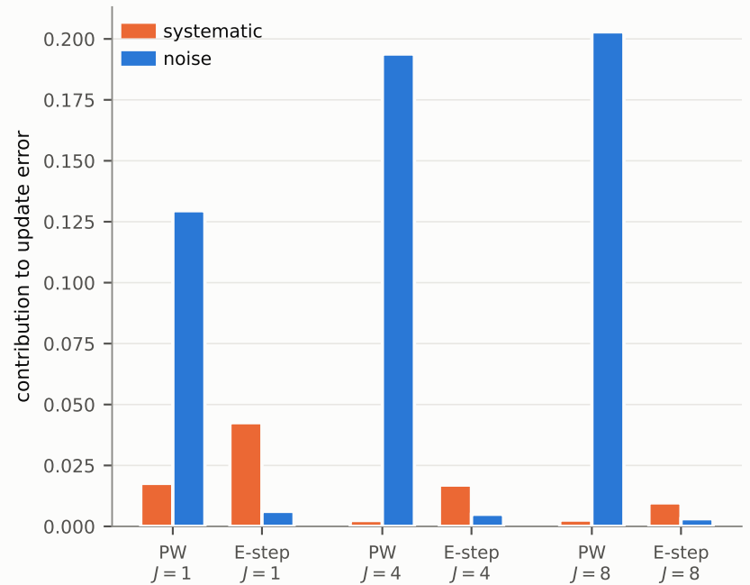
C Systematic vs noise, by operator
