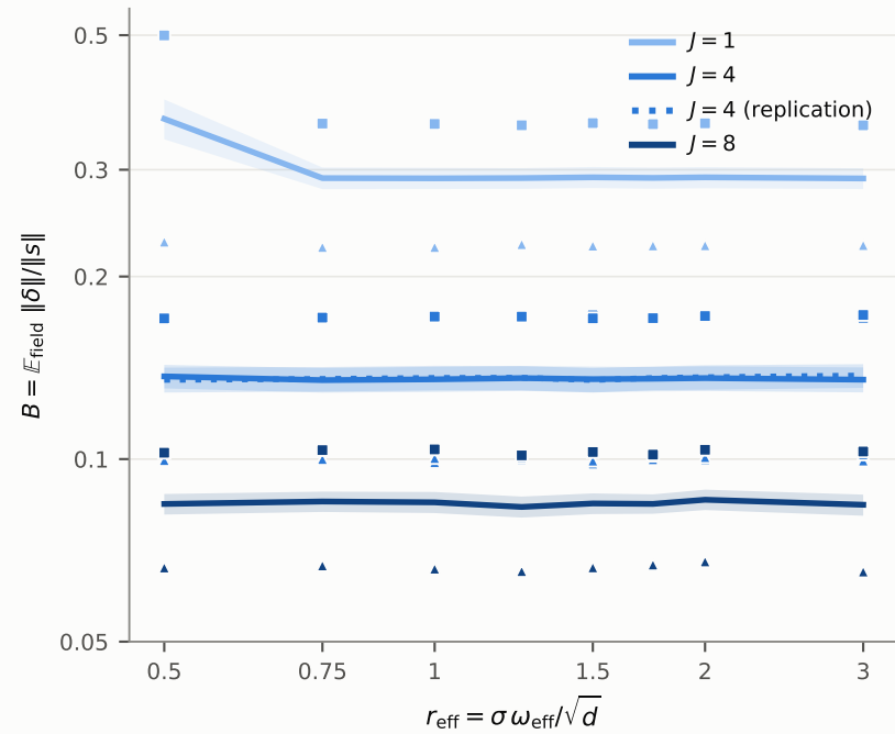
A E-step systematic displacement
