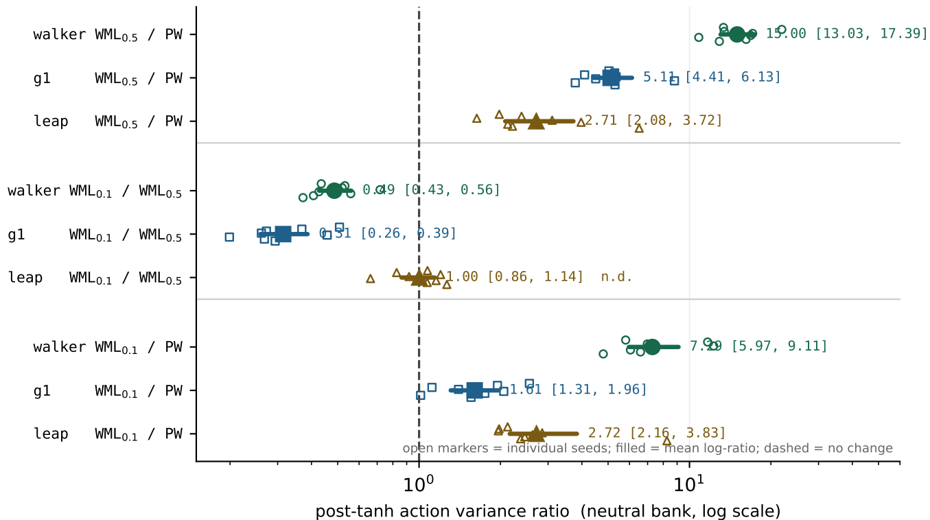
Post-tanh action-distribution geometry: all 8 seeds and paired bootstrap 95% CI
