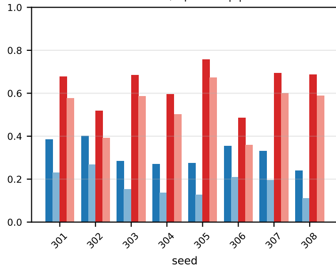
LEAP d=16 WML>PW in 8/8 pairs at |a|>0.95
