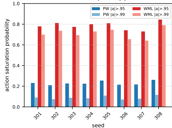
WalkerRun d=6 WML>PW in 8/8 pairs at |a|>0.95
