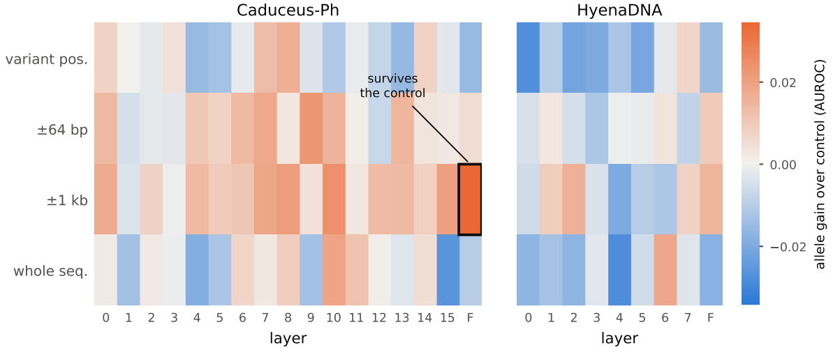
Figure 2: Allele signal by layer and summary window, for both frozen models. Colour is the gain of a nonlinear probe on e_{\text{alt}} - e_{\text{ref}} over the same probe on a random-allele control, so 0 means the probe was reading local context rather than the variant. F is the pooled final-layer state. Warm cells concentrate in the local windows and only one (Caduceus, final layer, \pm 1 kb) clears its control by a margin; it is still below the floor, and the ref_copy swap changes nothing there.
