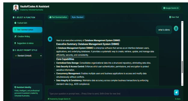
4. Text Summarization
