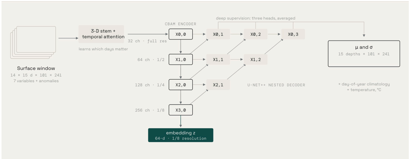
Figure 2. Architecture of the Sylithe Ocean Model. A 15-day window of 14 surface channels passes a 3-D stem with temporal attention and a CBAM encoder whose deepest level, projected to 64 channels, is the ocean-state embedding. The U-Net++ decoder with dense skip paths and deep supervision outputs a mean and an uncertainty at 15 depths, added to the day-of-year climatology.
