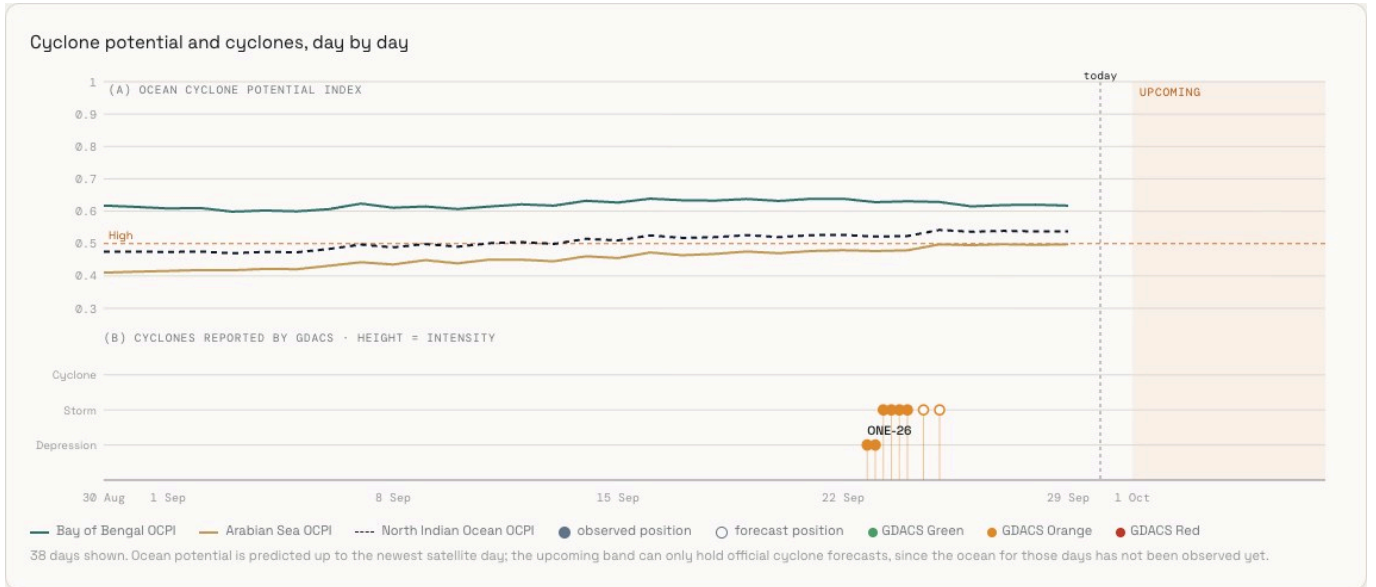
Figure 18. Live cyclone panel, 30 August – 7 October 2026. (a) OCPI of each basin's area-mean conditions over the predicted days, with a persistence outlook and today's High hotspots in the upcoming band. (b) Cyclones reported by GDACS: ONE-26 in the Bay of Bengal (solid: observed, hollow: forecast).
