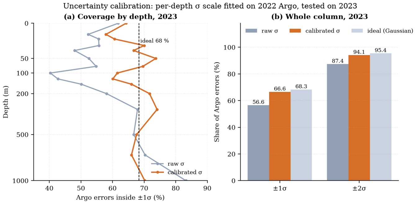
Figure 21. Uncertainty calibration fitted on 2022 Argo and tested on 2023: (a) coverage of \pm 1\sigma by depth, (b) whole column.
