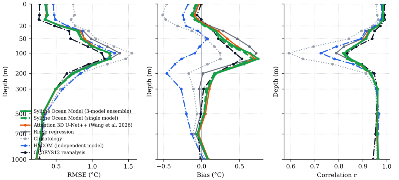
Figure 6. The same scores against independent Argo profiles. GLORYS12 is best near the surface because it assimilates these floats; below 200 m the Sylthe Ocean Model matches or beats it.
