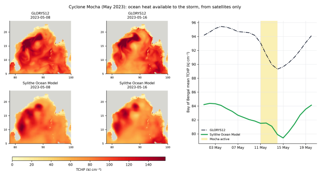
Figure 16. Tropical cyclone heat potential from the reconstruction and from GLORYS12 around Cyclone Mocha (May 2023).
