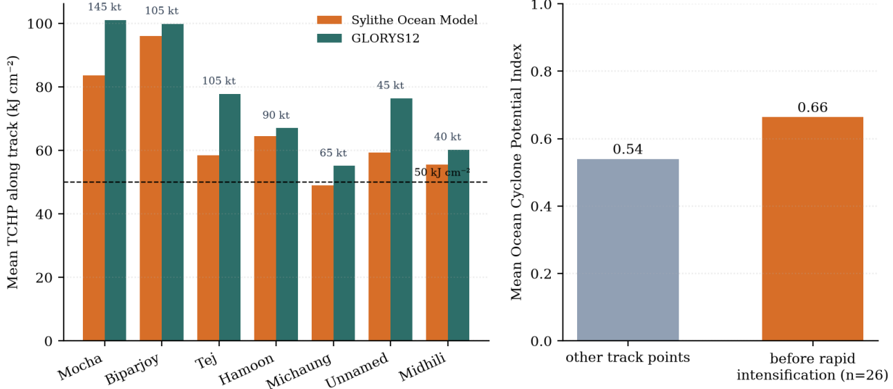
(a) Heat potential along tracks · r = 0.88 , bias -9.9 (b) OCPI before rapid intensification · AUC 0.70
