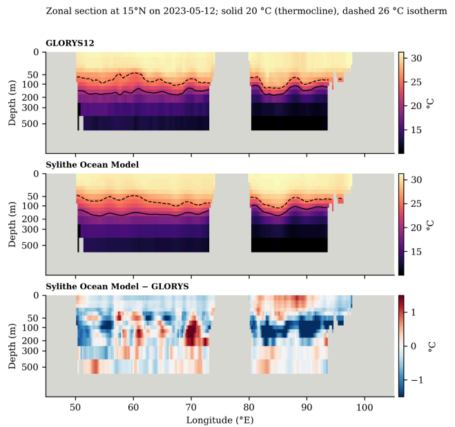
Figure 15. Vertical temperature section through the Bay of Bengal on 12 May 2023: reconstruction and GLORYS12.
