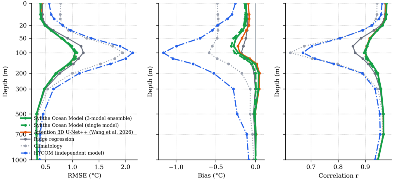
Figure 5. RMSE, bias and correlation by depth against GLORYS12 over every day and ocean cell of 2023, for all methods. The Sylthe models and the published architecture track each other closely and are far better than HYCOM and climatology in the thermocline.
