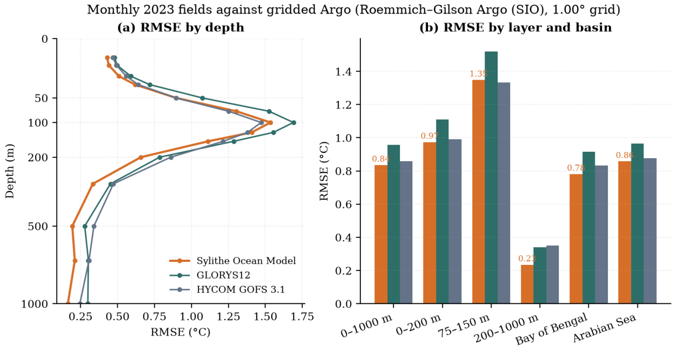
Figure 20. Monthly 2023 fields against Roemmich–Gilson gridded Argo: (a) RMSE by depth, (b) RMSE by layer and basin.
