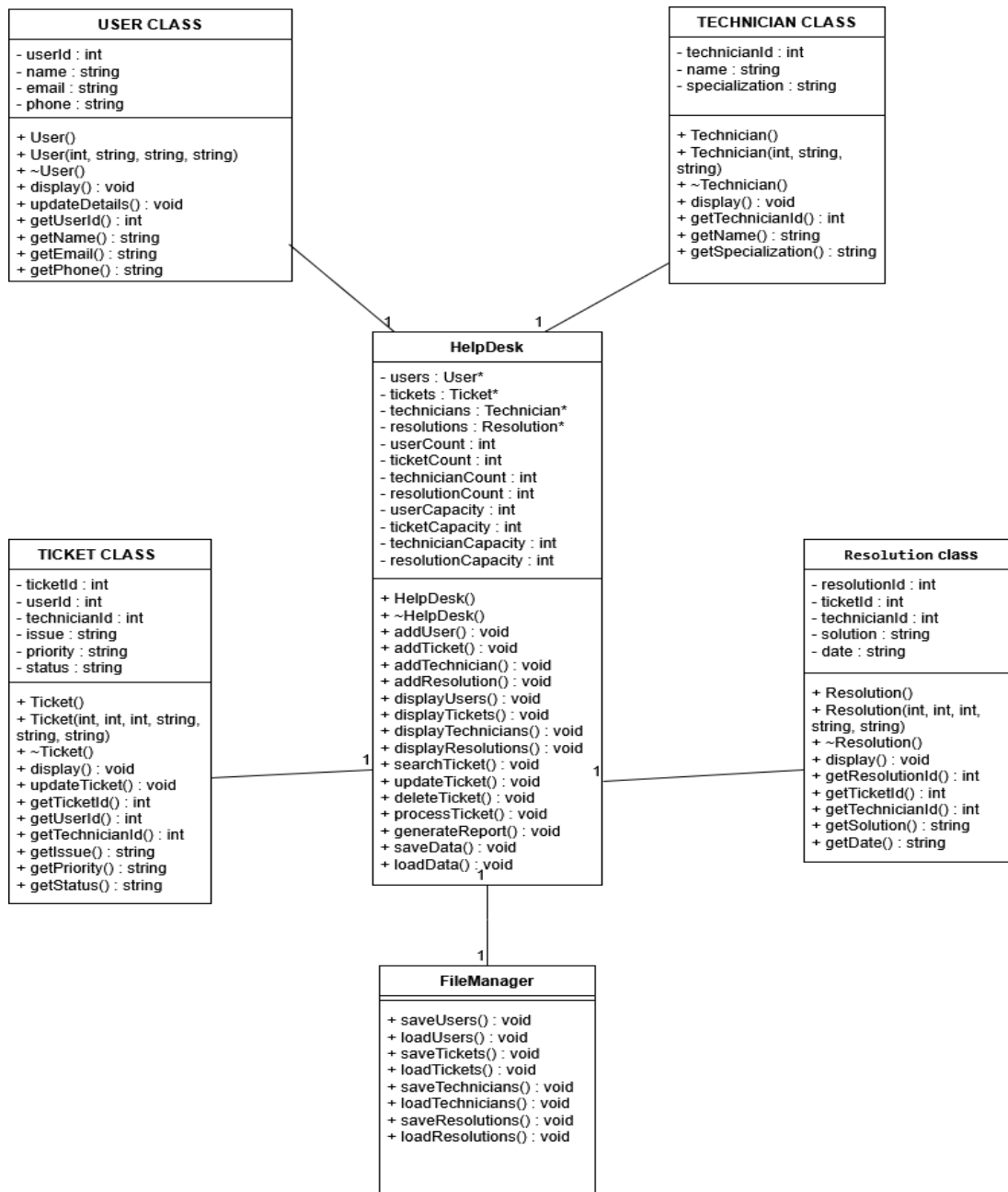
Figure 4: Class Diagram
