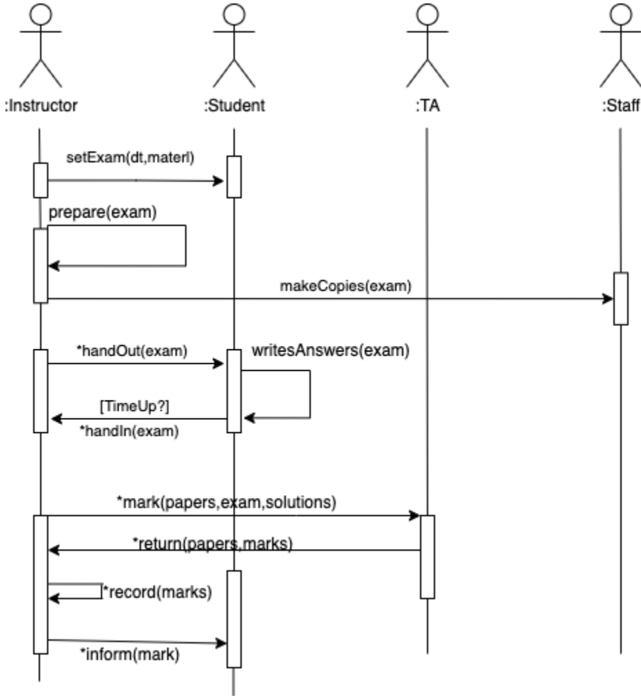
Q.2 Sequence diagram
