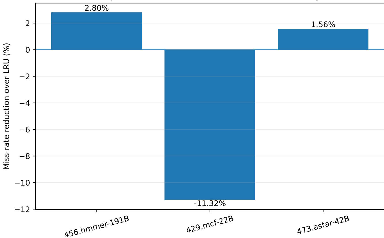
Hawkeye LLC miss-rate reduction over LRU - 16-way LLC
