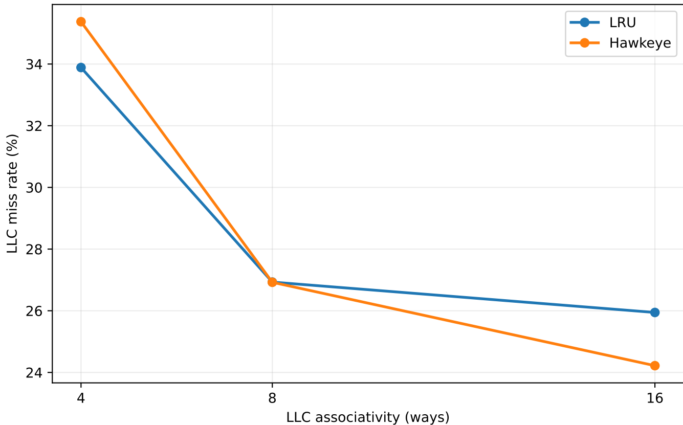
LLC miss rate vs. associativity - 456.hmmmer-191B
