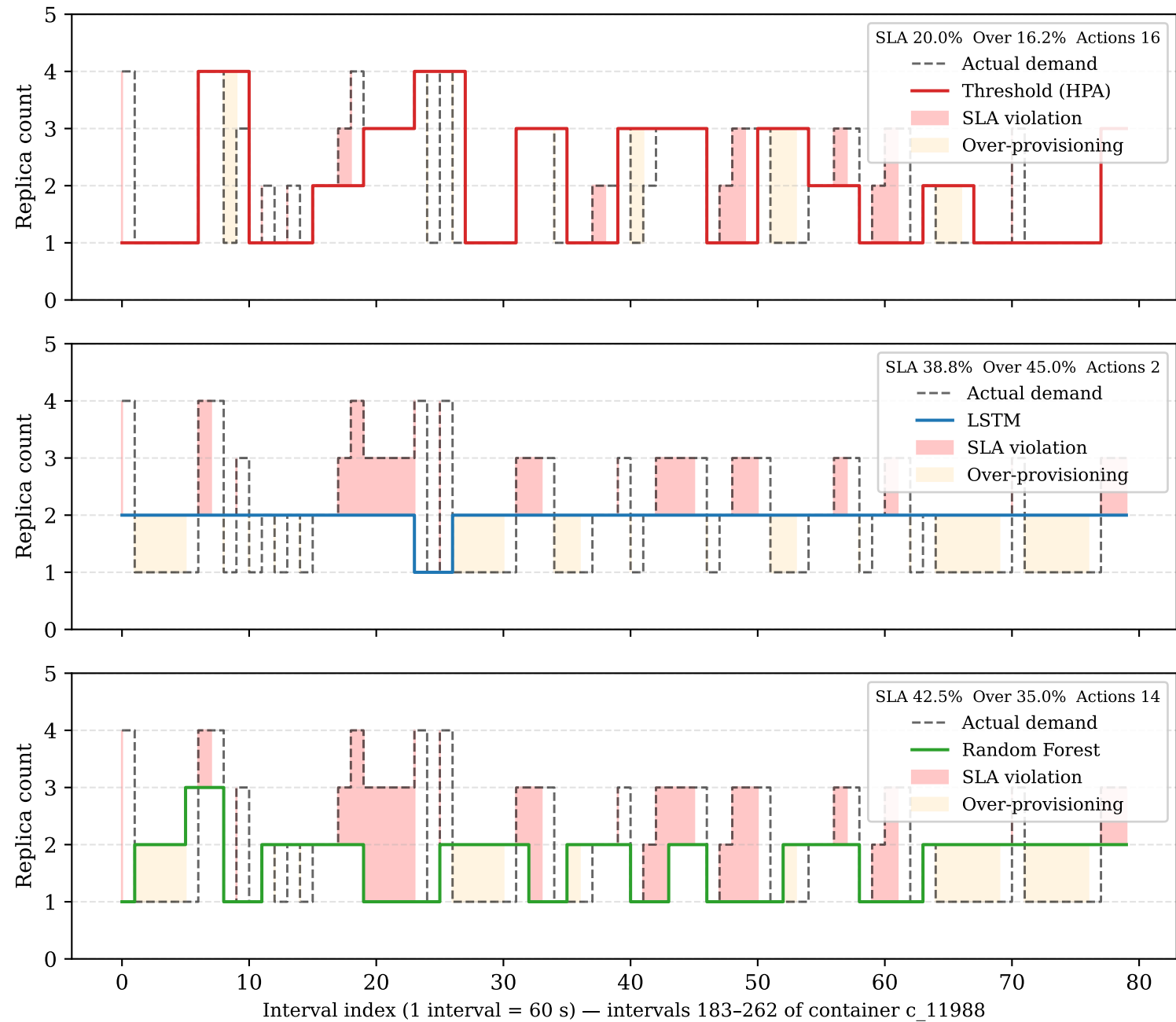
Reactive vs Proactive Scaling — HPA, LSTM, and Random Forest (highest-variance 80-interval window, container c_11988)
