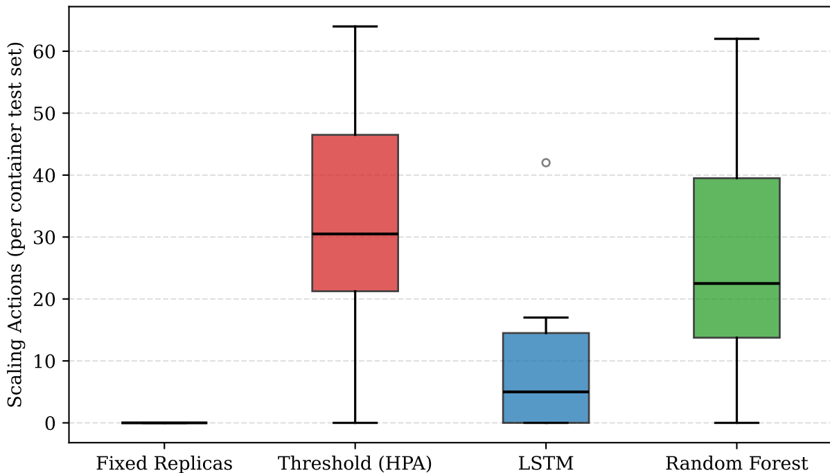
Scaling Action Count Distribution Across Containers
