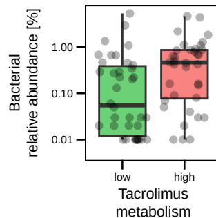
Faecalibacterium
