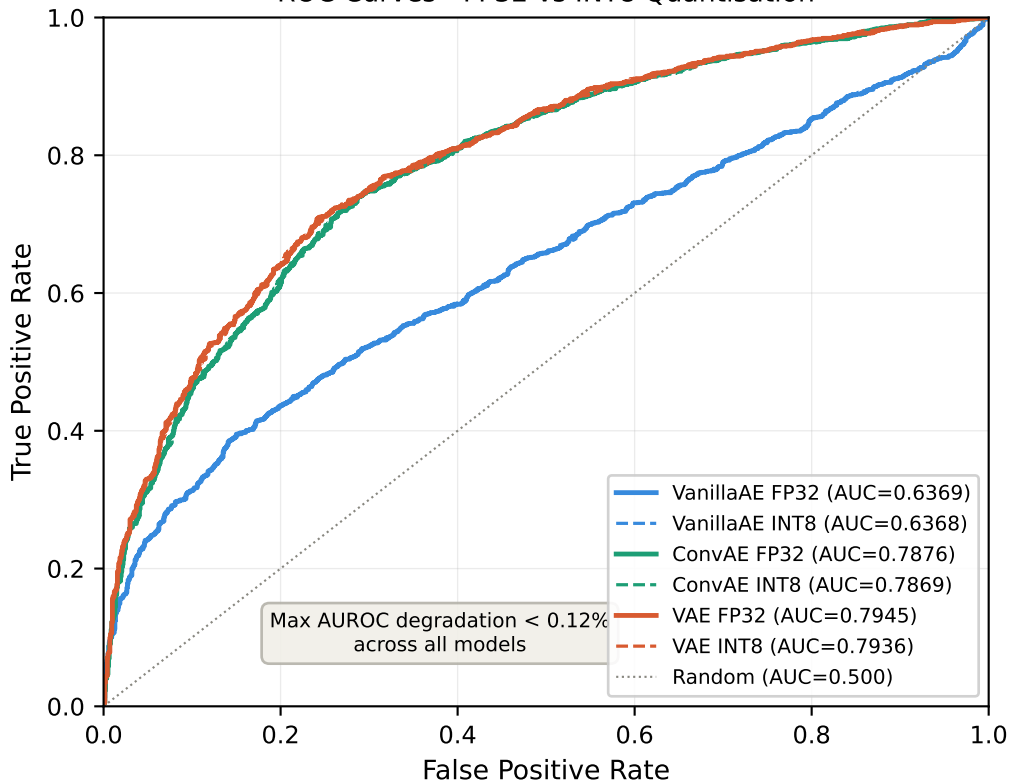
ROC Curves - FP32 vs INT8 Quantisation
