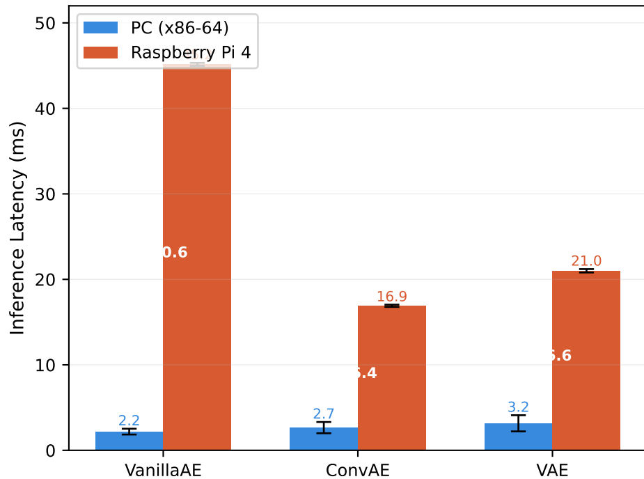
(a) FP32 Latency: PC vs Pi4
