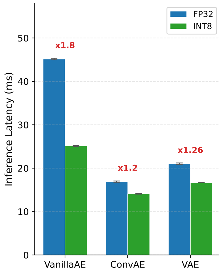
(b) Pi4 Inference Latency
