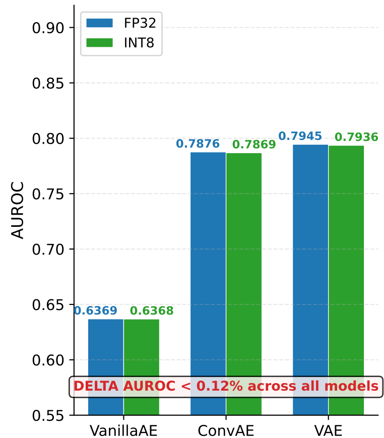
(c) AUROC Degradation
