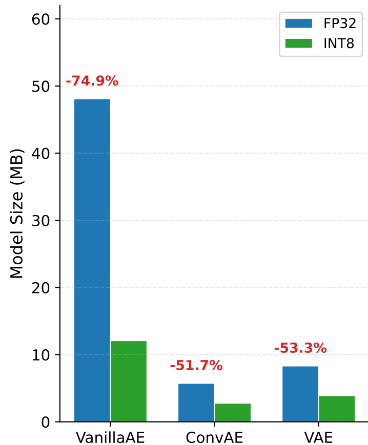
(a) Model Size Reduction
