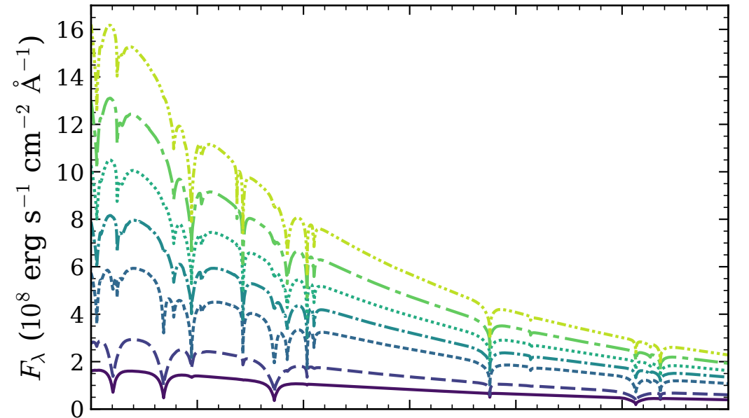
Optical hydrogen and helium features
