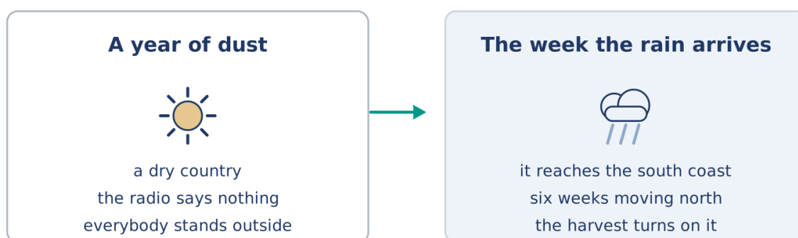
Figure 12.35 · A year of dust, and the week the rain arrives.
