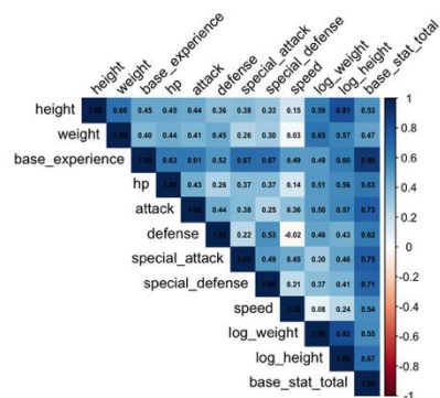
Correlation Matrix
