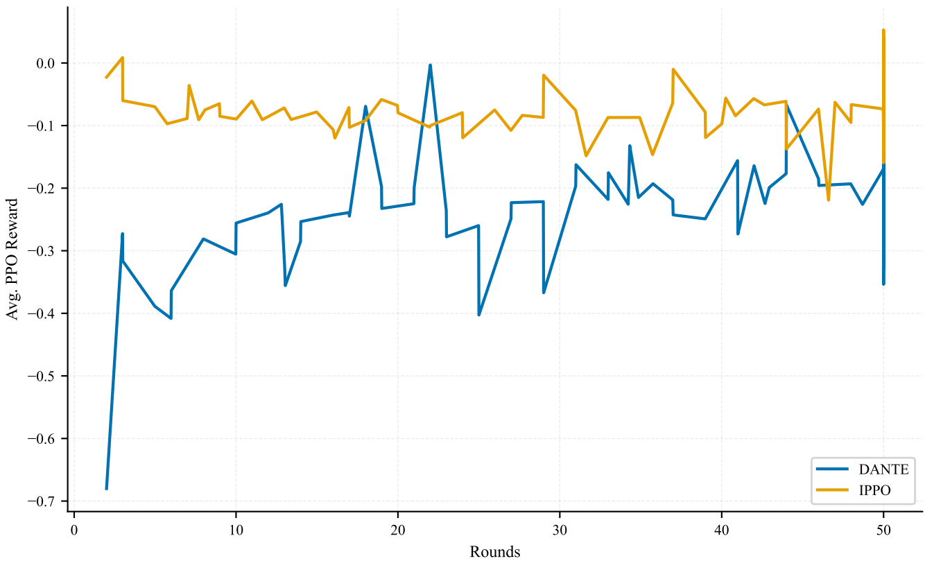
PPO Reward vs Rounds
