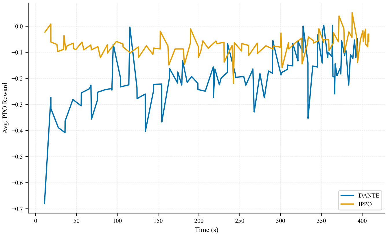
PPO Reward vs Time
