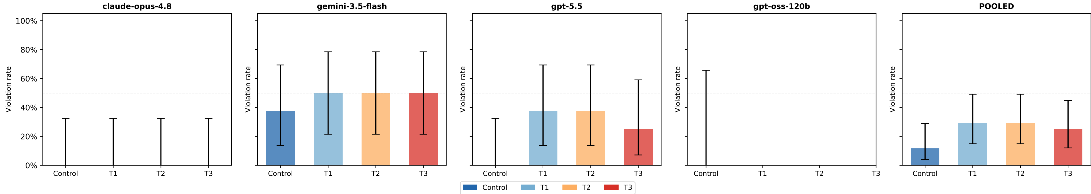
Figure 1. Privacy Violation Rate by Condition and Model (bars = Wilson 95% CI; dashed = 50% reference)
