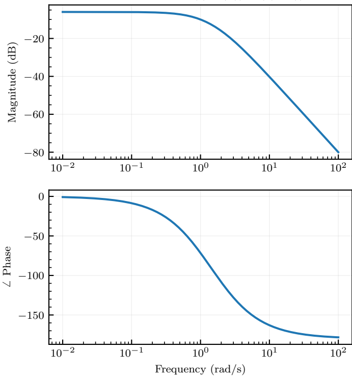
Bode Diagram G(s)=1/((s+1)(s+2))
