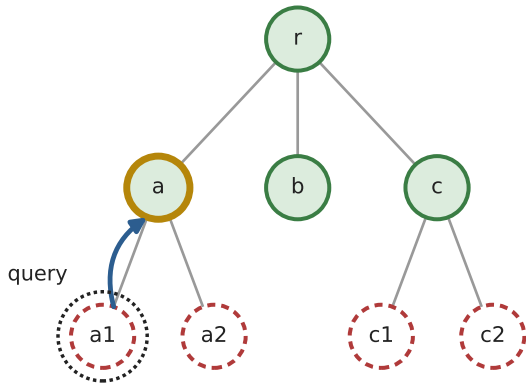
(b) Miss reconstruction
