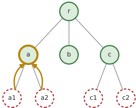
(a) Eviction and summarisation
