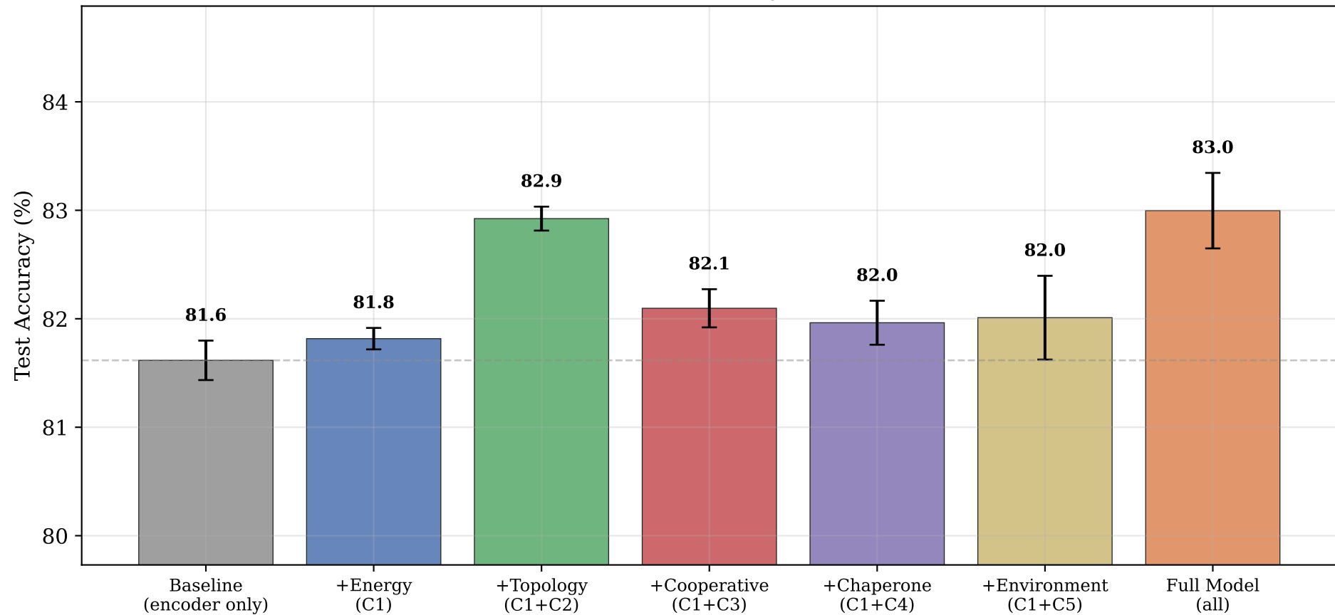
FoldFlow Ablation Study — CIFAR-10
