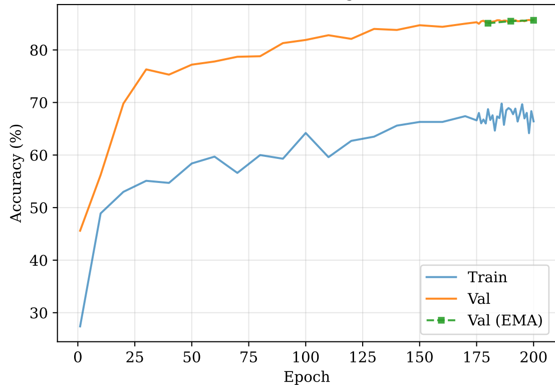
CIFAR-10 Training Curves
