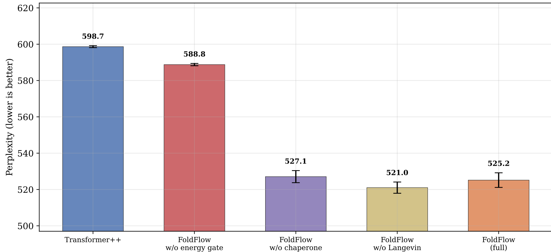
WikiText-2 Language Modeling — Component Ablation
