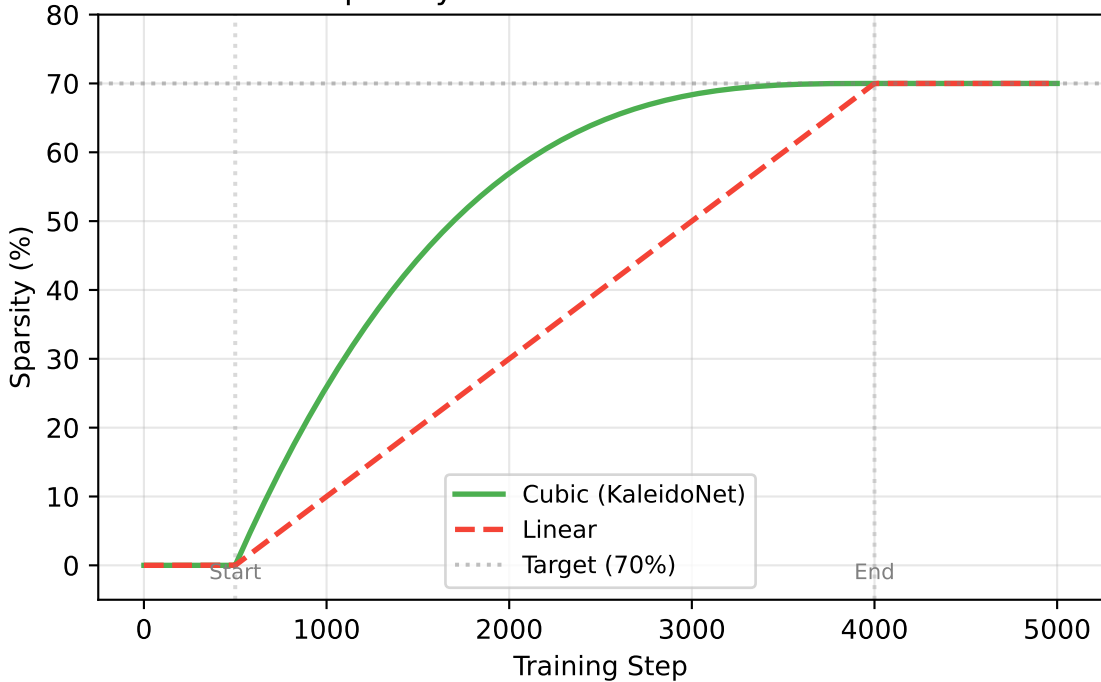
Sparsity Schedule: Cubic vs Linear
