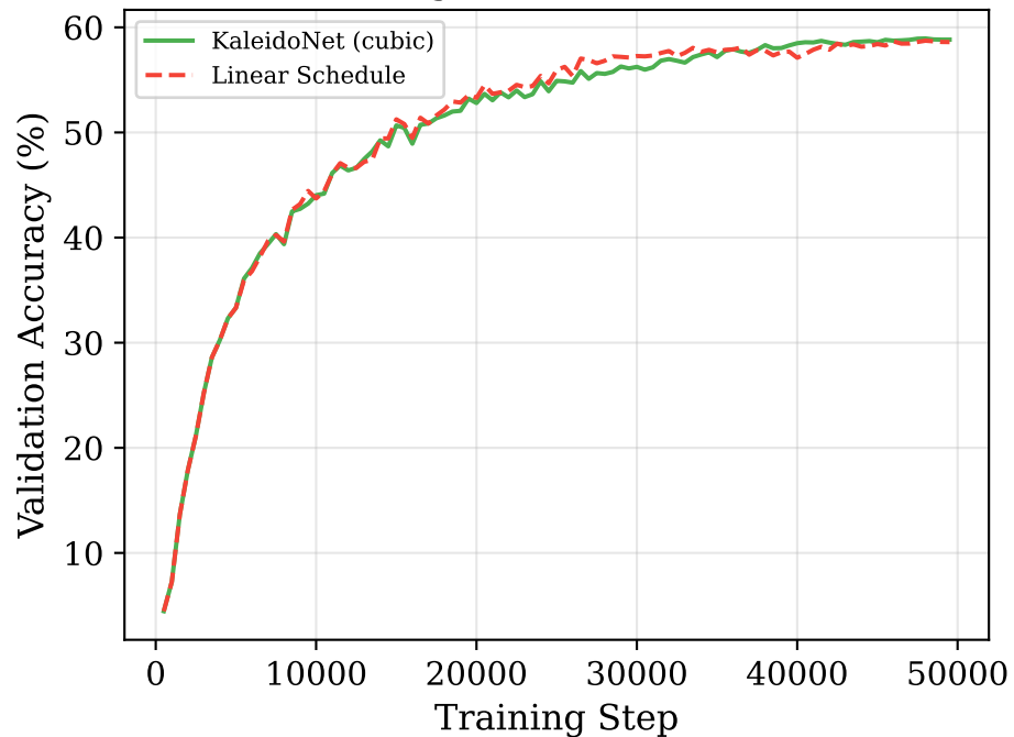
Convergence on CIFAR-100
