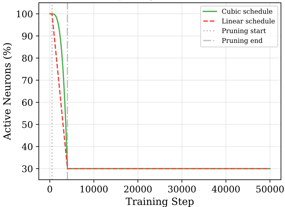
Sparsity Schedule
