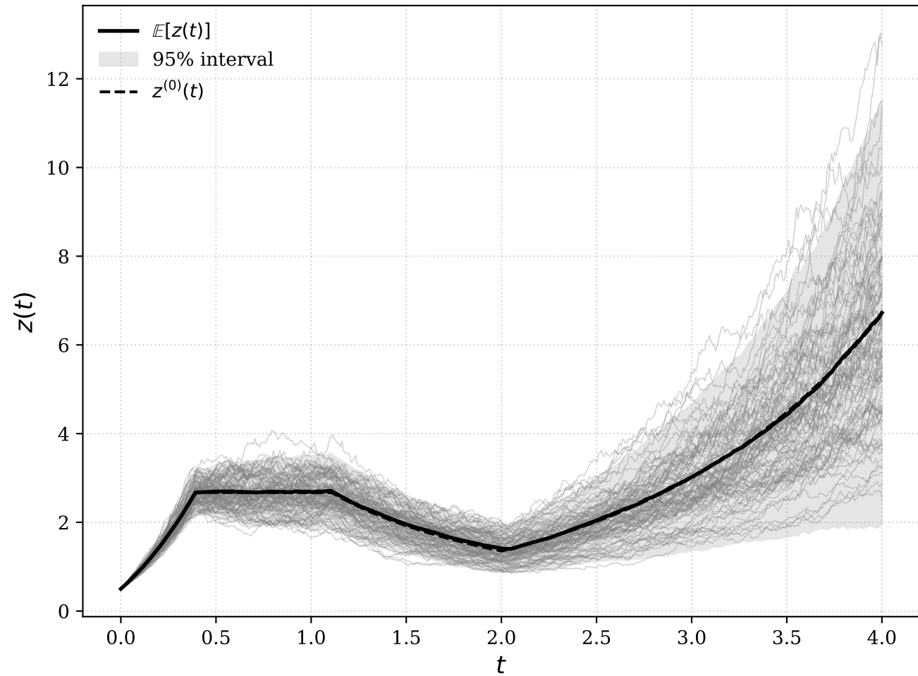
Stochastic trajectories of z(t)
