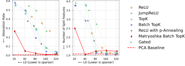
Figure 6. Feature absorption and splitting. Matryoshka SAEs significantly reduce feature absorption and splitting compared to baselines.
