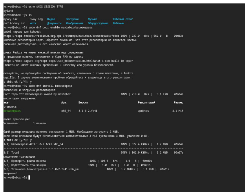
Рис. 6: native messaging
