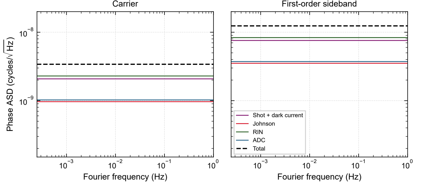
FIG. 3. Calculated carrier and first-order sideband readout noise for the stated bright-beam operating point. The model uses a 50\ \Omega load at 300 K, 100 nA dark current, and white fractional intensity noise of 9 \times 10^{-9}/\sqrt{\text{Hz}} , with the two beams' additive intensity noise summed coherently. The assumed current-to-voltage gain at each ADC is 50/\sqrt{3}\ \text{V/A} , with a 1 V full-scale span, 14 bits and 2 GS/s. The ADC curve is ideal quantization noise. The calculation assumes linear detection and adequate filtering before sampling and decimation; it does not include a measured receiver or phasemeter noise floor.
